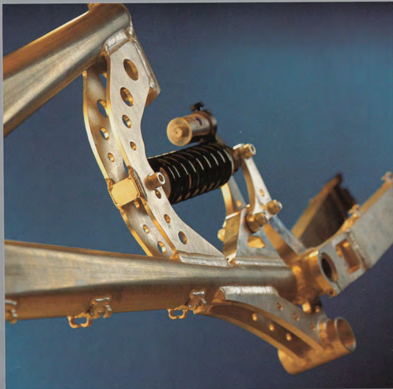
Welded perfection. An RM9 frame ready for powder coating.
