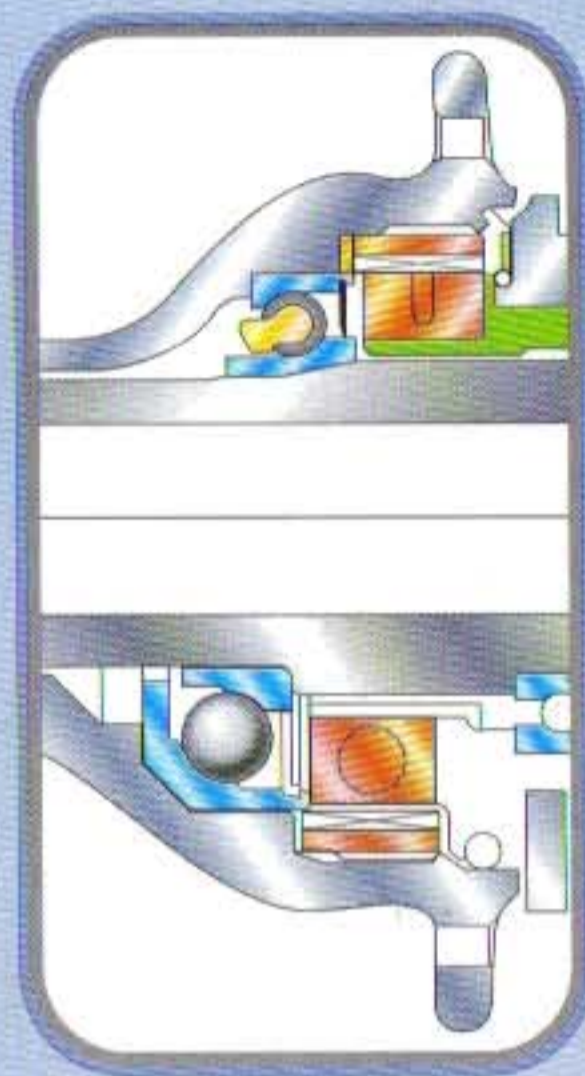
New Record '99 rear hub
