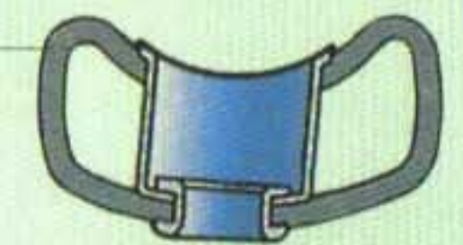
Cross-section of Climb-Dynamic wheels for tubular tires.
