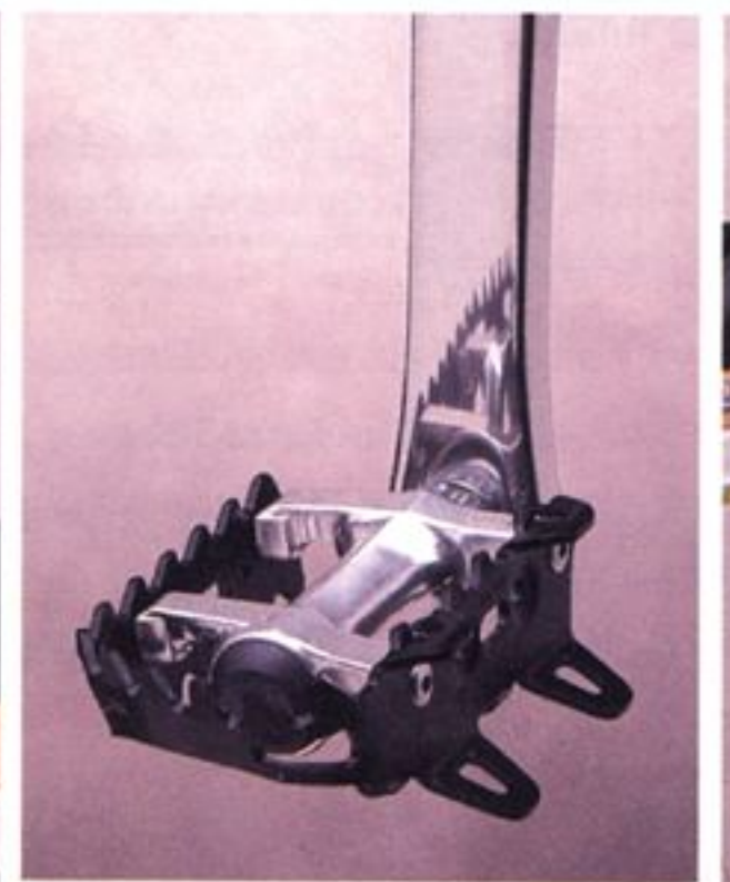
Tioga SureFoot pedals are toe clip compatible and feature sealed, Chromoly spindles.
