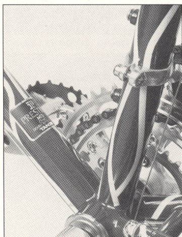
Note the surface mounted water bottle bosses. This reduces the number of holes drilled into the frame. Wiggle Wire paint finish.
