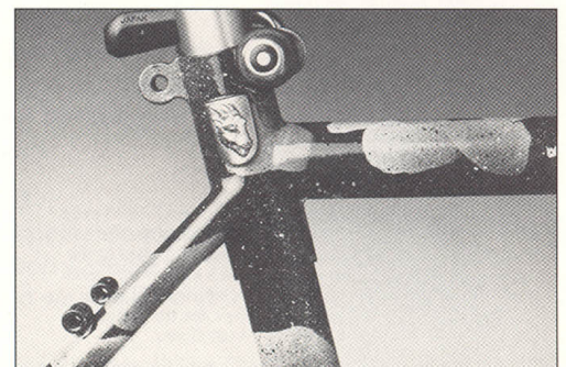
The reinforced seatlug collar, not only offers a stronger seatlug, but lets you attach your Hite-Rite™ without interfering with your quick release seatpost binder bolt.
