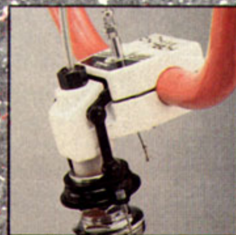
SR Spintech stem provides thru-stem cable routing.
