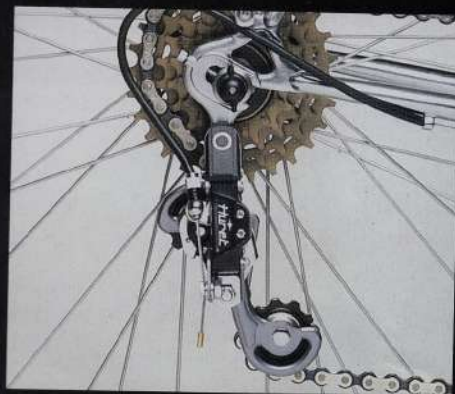
Huret titanium-bodied Duopar gear
